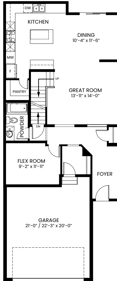
MAIN - 1,052 SF
