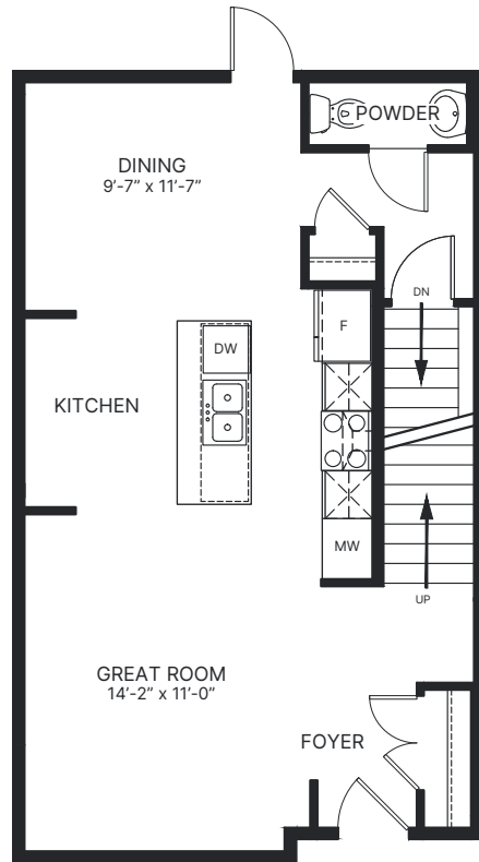
MAIN - 662 sq. ft.
